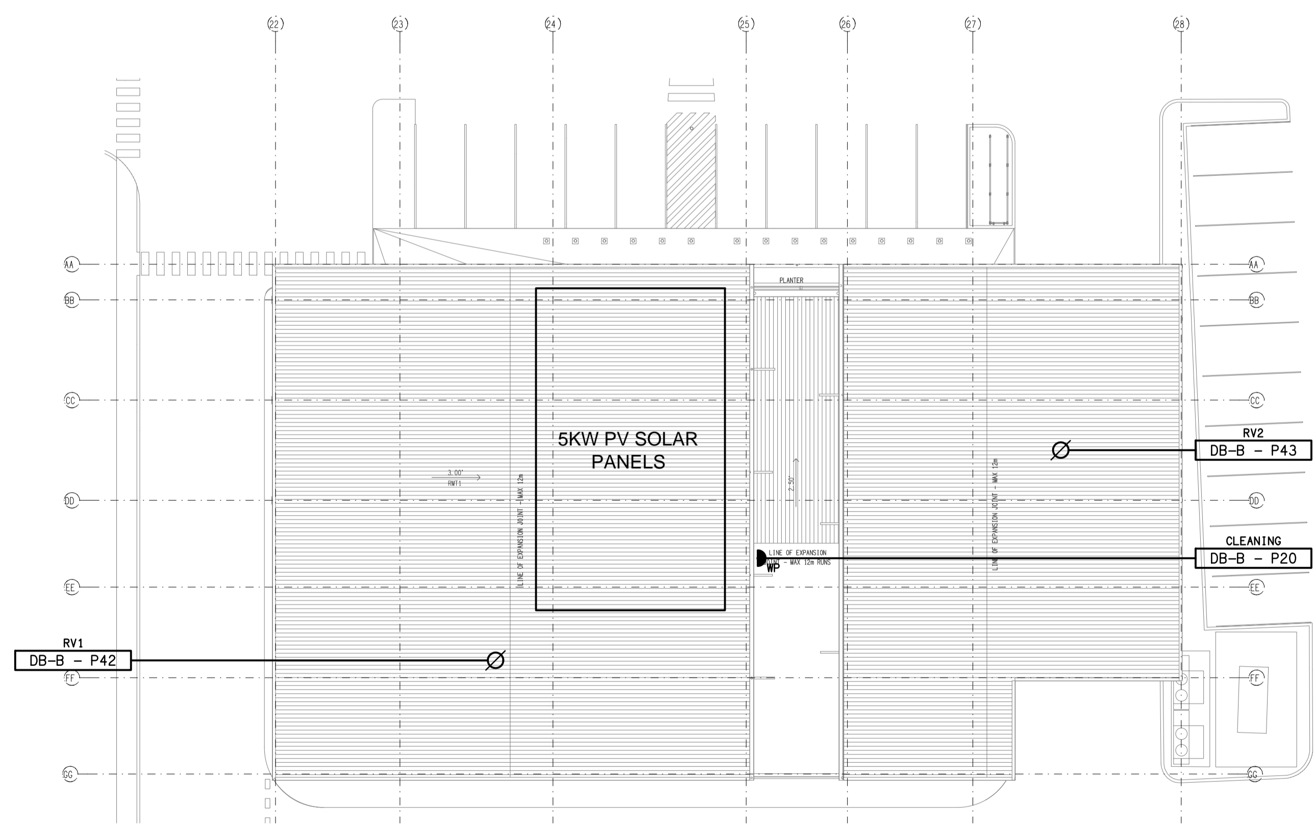
BOTTLE SHOP ROOF PLAN SCALE 1:200
